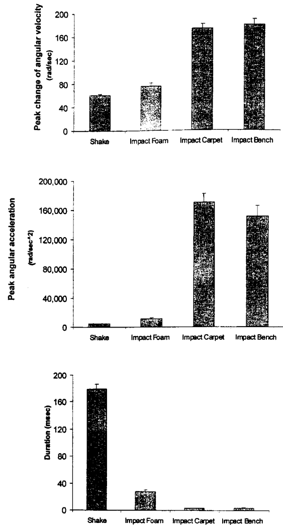
FIG. 5. Bar graphs showing the inflicted \Delta\dot{\theta}_{\max} (upper), \dot{\theta}_{\max} (center), and \Delta t (lower) for shakes and impacts against different surfaces.
